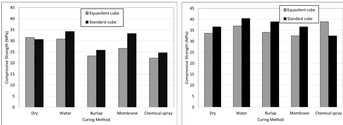
Figure 8: Comparison between Equavilat and Standard Cube Compressive Strength for 350 kg/m 3 Concrete Mixes Cured in Various Methods
