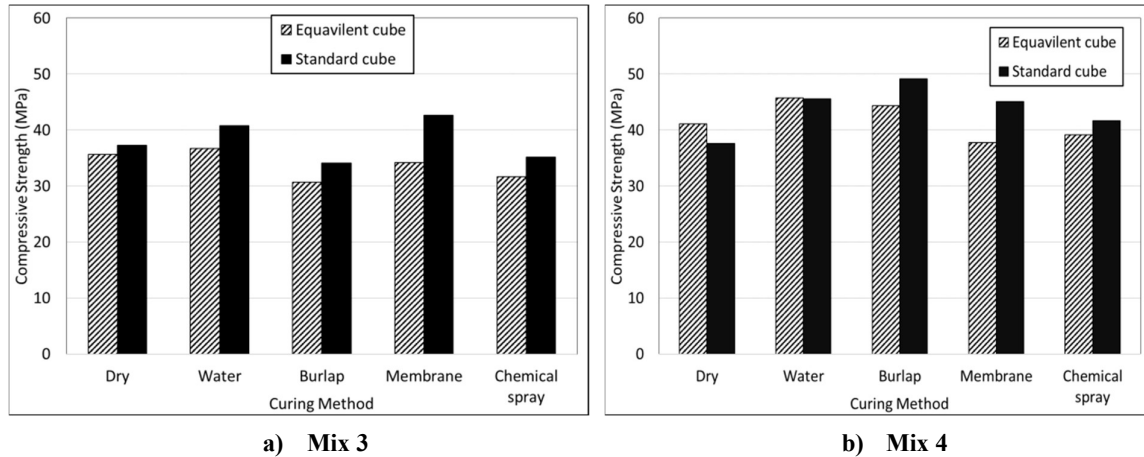
Figure 9: Comparison between Equivalent and Standard Cube Compressive Strength for 450 kg/m 3 Concrete Mixes Cured in Various Methods
