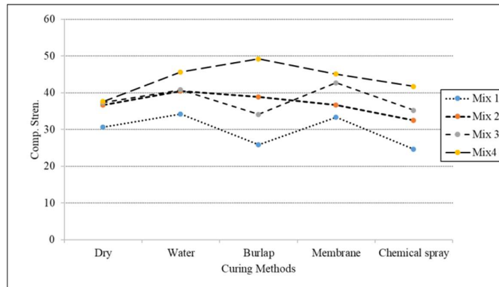
Figure 6: Compressive Strength for Concrete Mixes Cured in Various Methods at 28 days
