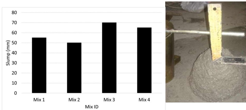
Figure 3: Slump Results
