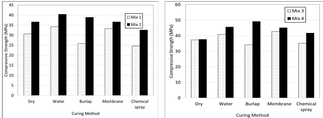
a) 350Kg/m 3 b) 450Kg/m 3 Figure 5: Compressive Strength for Concrete Mixes Cured in Various Methods at 28 days
